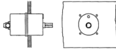
Through console installation with short shaft
